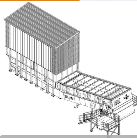
Trucks surface feeder
